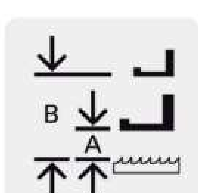
Top feed stroke (A) and fabric clearance (B)
