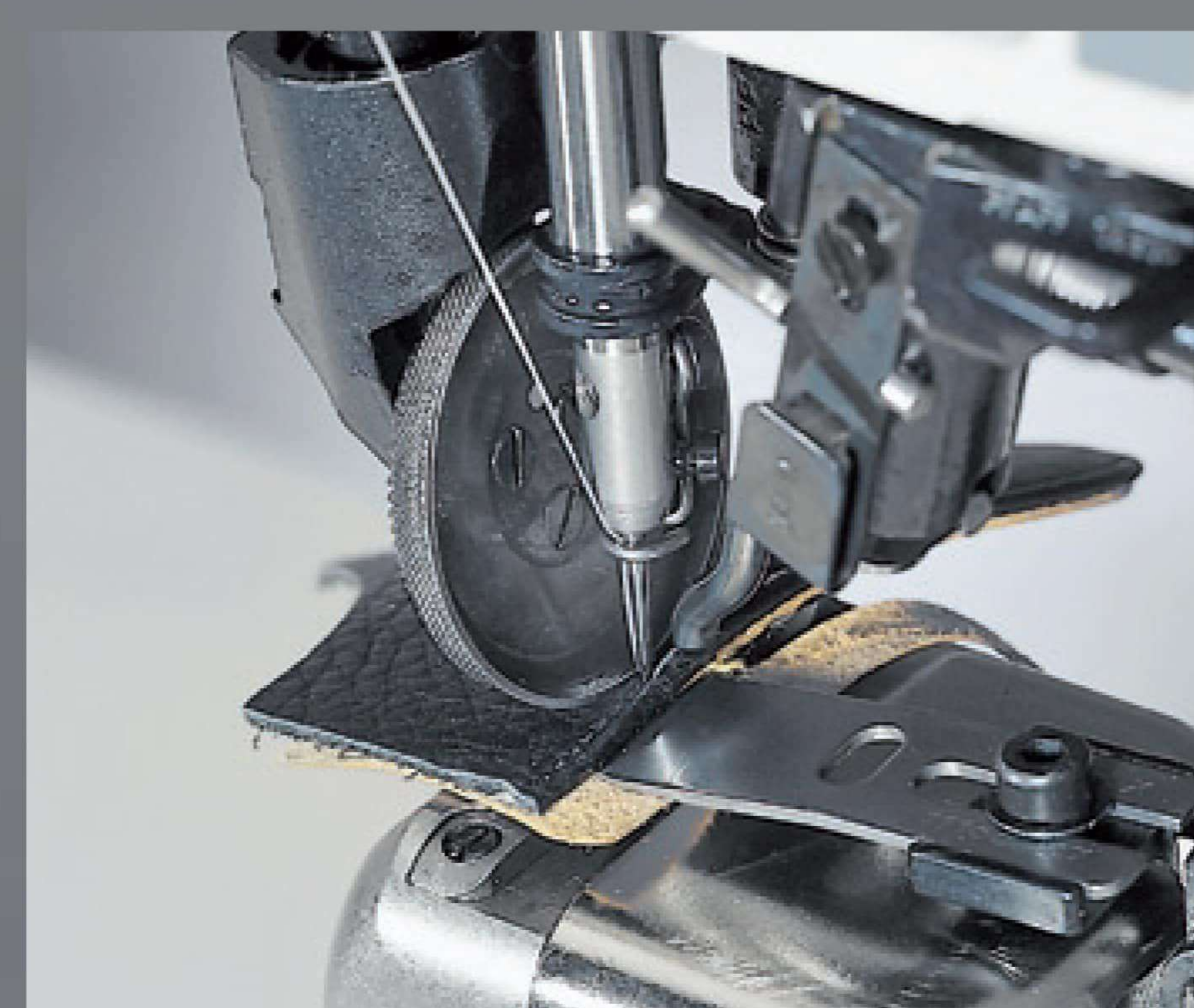
PFAFF 591/ 1591 with edge trimming mechanism
