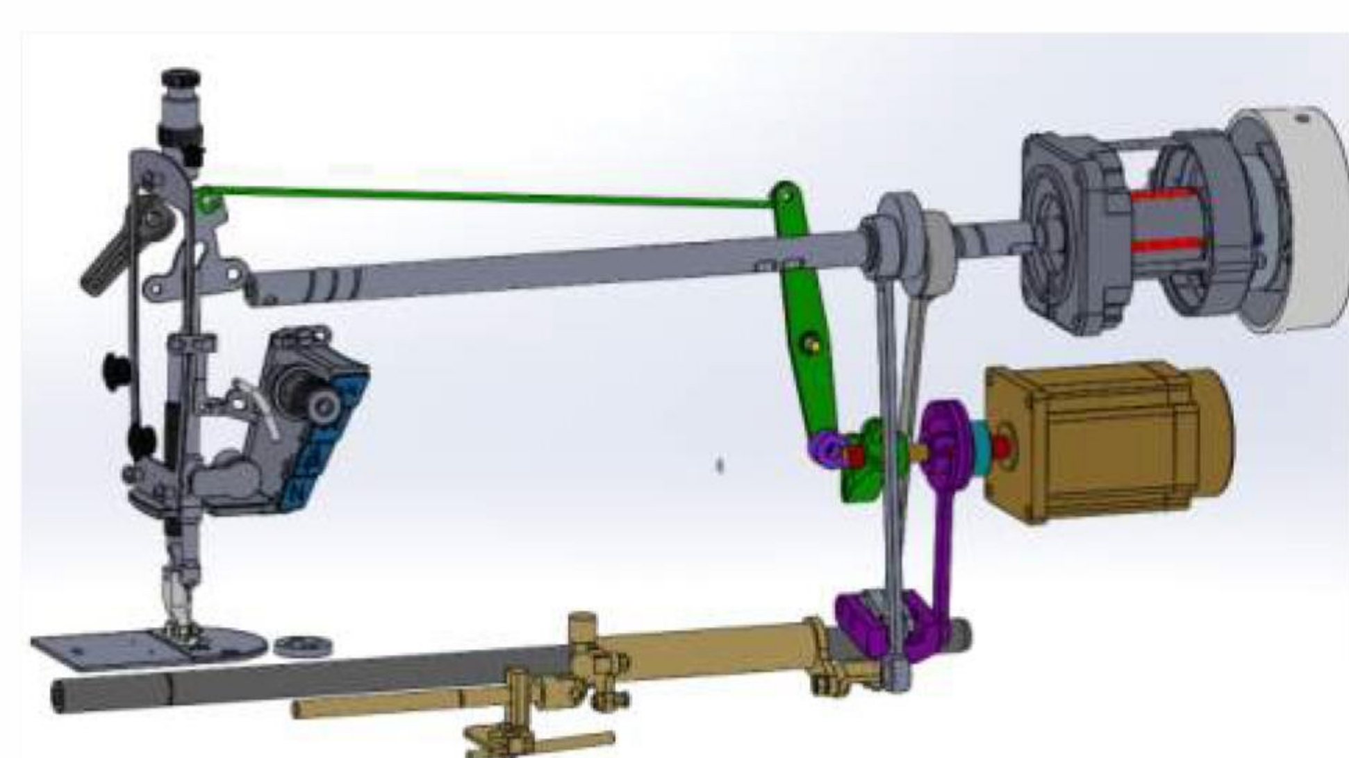
步进电机一拖四控制：针距、倒缝、剪线、抬压脚、松线 Step motor control 4 automatic functions: Needle gauge, reverse feeding, trimming, pressure foot lift.
